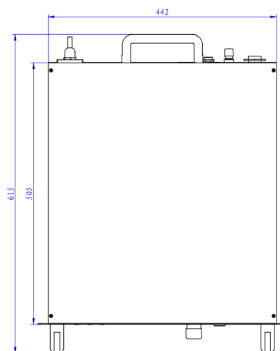
Left View
